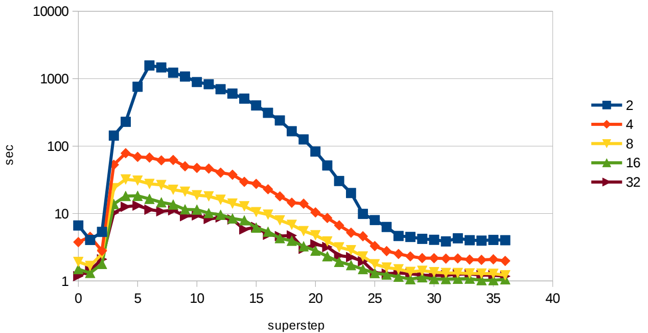
Fig. 2. Time distribution over supsteps (y — log scale).
